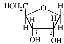
2-Deoxy-D (-)-Ribofuranose
