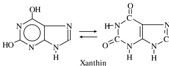
Acid Uric
