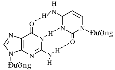
Cặp Guanin-Cytosin
