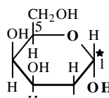
2-Deoxy-D- \alpha - Glucopyranose
