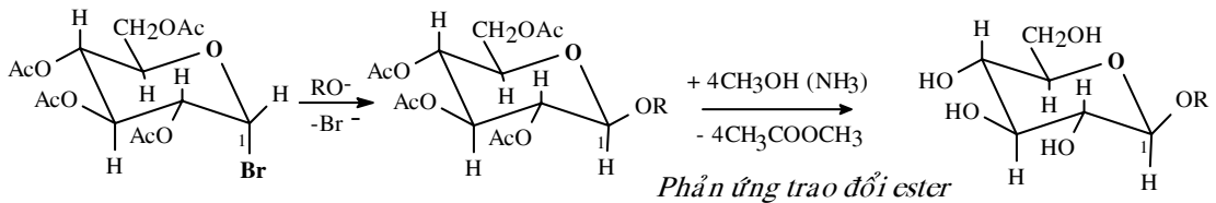
1-Brom-2,3,4,6-tetra-acetyl- \alpha\text{-D-Glucopyranose}
