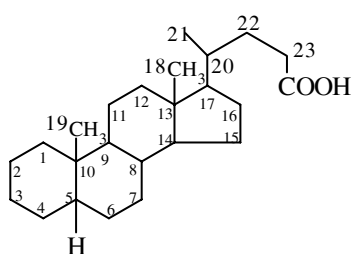
Acid Cholanic
