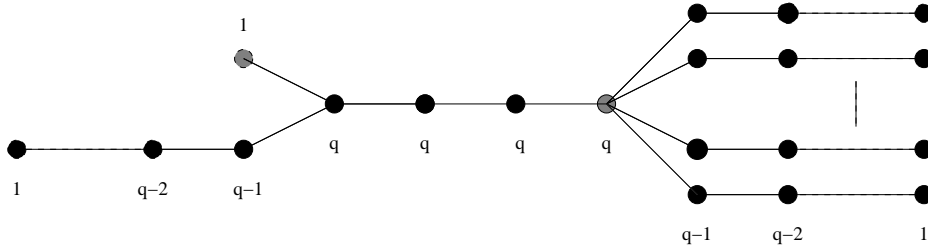
Figure 1: Dual graph of \psi^{-1}(\infty) with multiplicities
