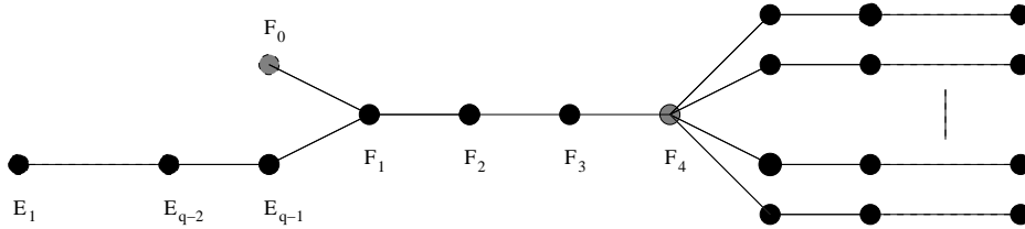
Figure 3: Dual graph of \psi^{-1}(\infty)
