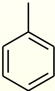
phenyl
