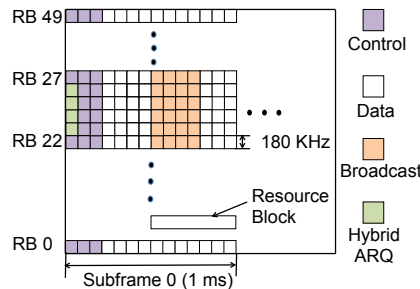
Figure 2: Physical Channels are mapped to well defined Resource Elements in the Grid.
