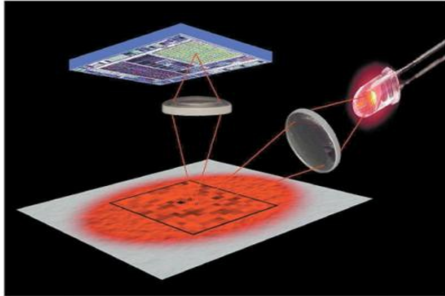
Figure 1. Optical mice illuminate an area of the work surface with an LED, to reveal a microscopic pattern of highlights and shadows. These patterns are reflected onto the navigation sensor, which takes pictures at a rate of 1500 images per second or more.
