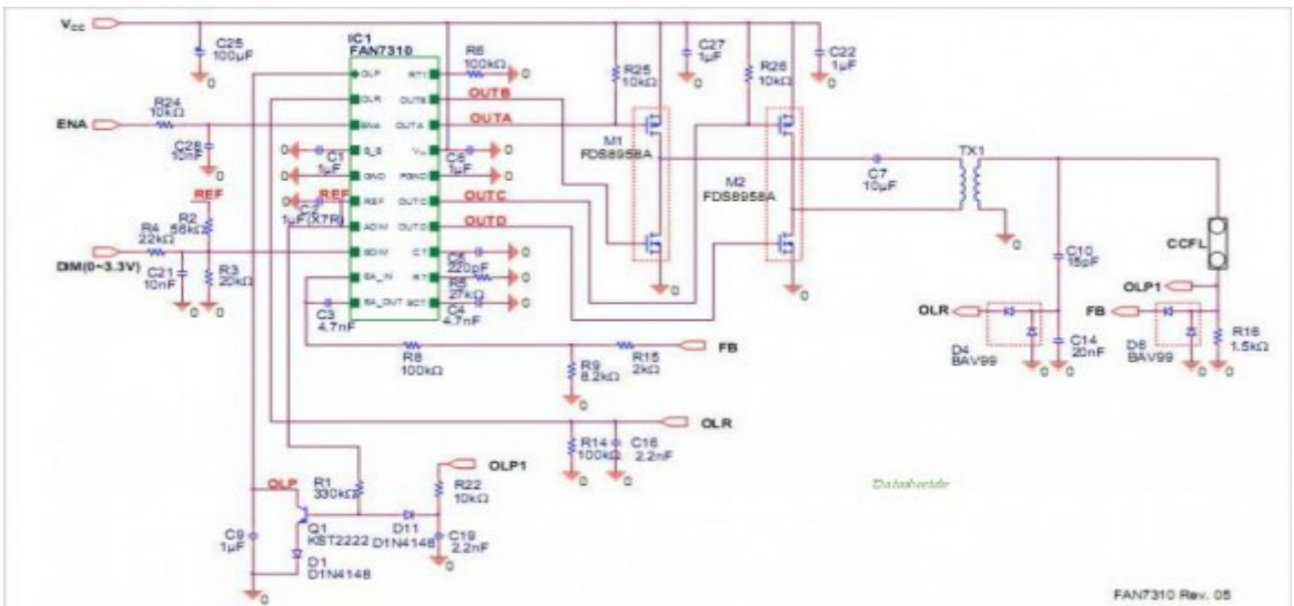
Figure 1. Application Circuit for CCFL
