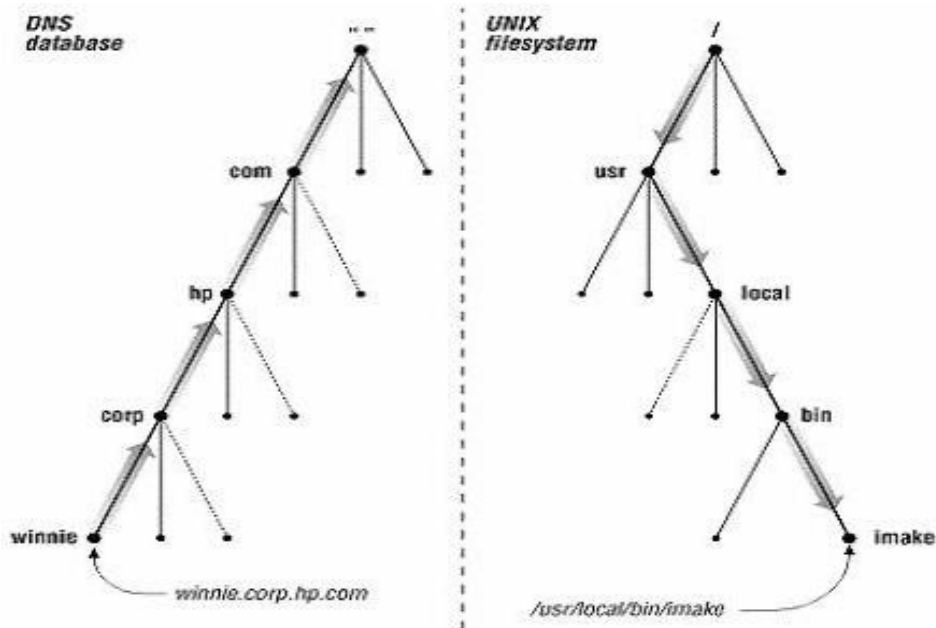
DNS database
