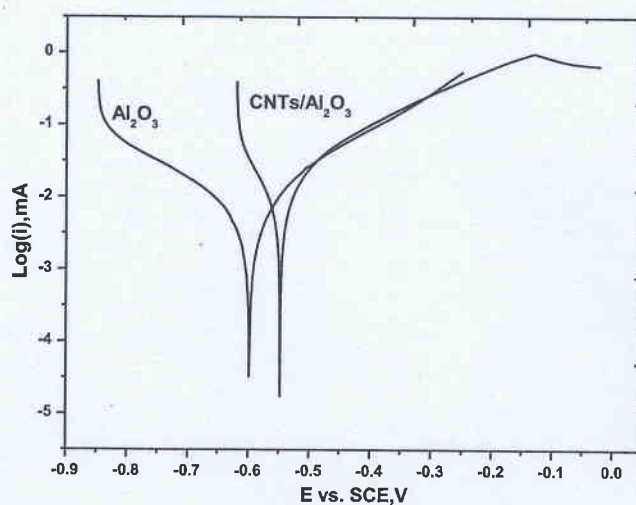
Figure 8. Polarization curves of Al_2O_3 and CNTs/ Al_2O_3 coatings measured in 3.5 % NaCl solution.
