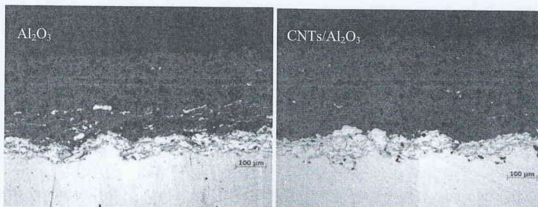
Figure 6. Cross-sectional structures of \text{Al}_2\text{O}_3 and \text{CNTs}/\text{Al}_2\text{O}_3 coatings.
