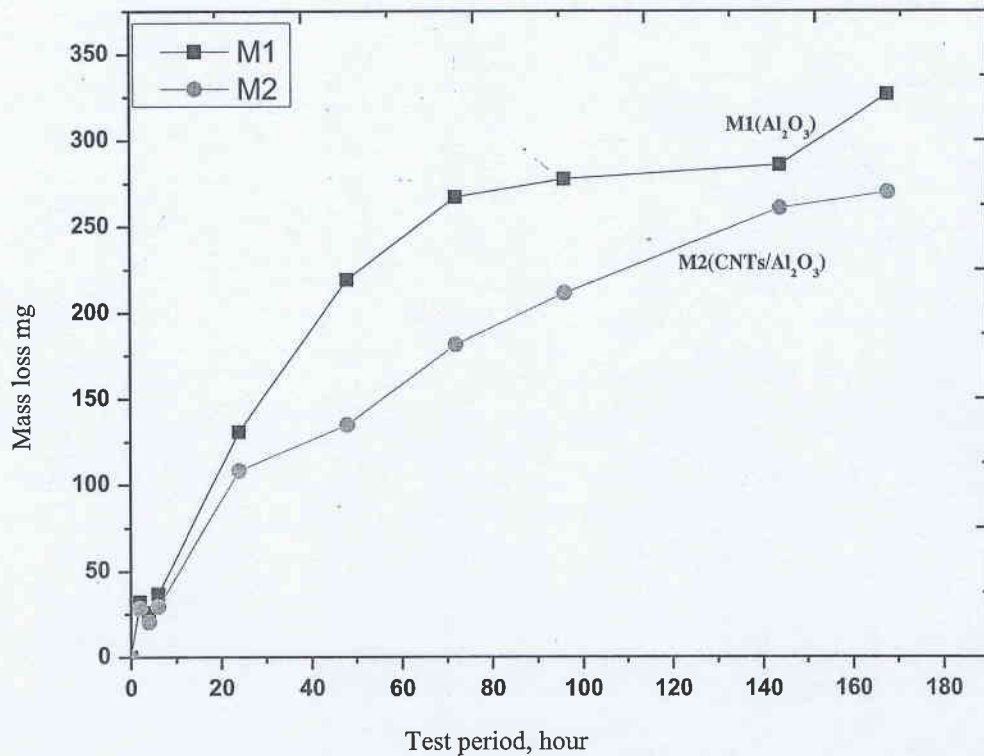
Figure 9. Erosion corrosion resistance of coatings.
