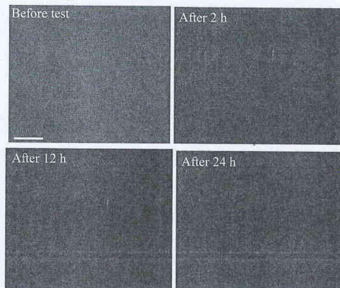
Figure 5. Surface change of CNTs/Al 2 O 3 coating during the salt spray test.
