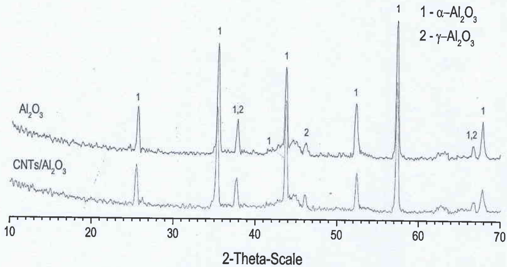
Figure 3. XRD of \text{Al}_2\text{O}_3 powder after mixing with CNTs.
