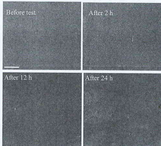
Figure 4. Surface change of Al 2 O 3 coating during the salt spray test.
