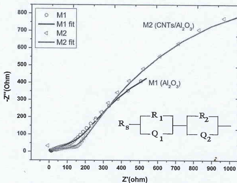
Figure 7. Nyquist diagram of Al_2O_3 and CNTs/ Al_2O_3 coating measured in 3.5 % NaCl solution.
