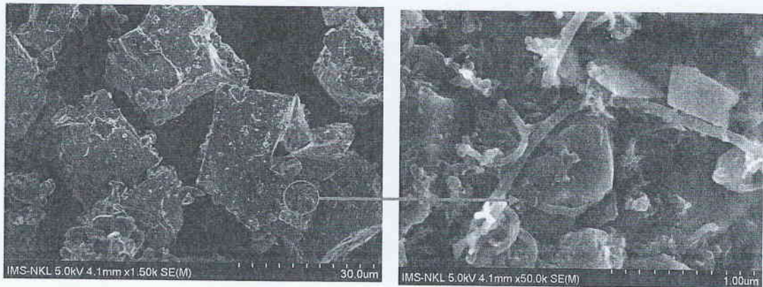
Figure 2. SEM image of \text{Al}_2\text{O}_3 powder after mixing with 1 % CNTs.
