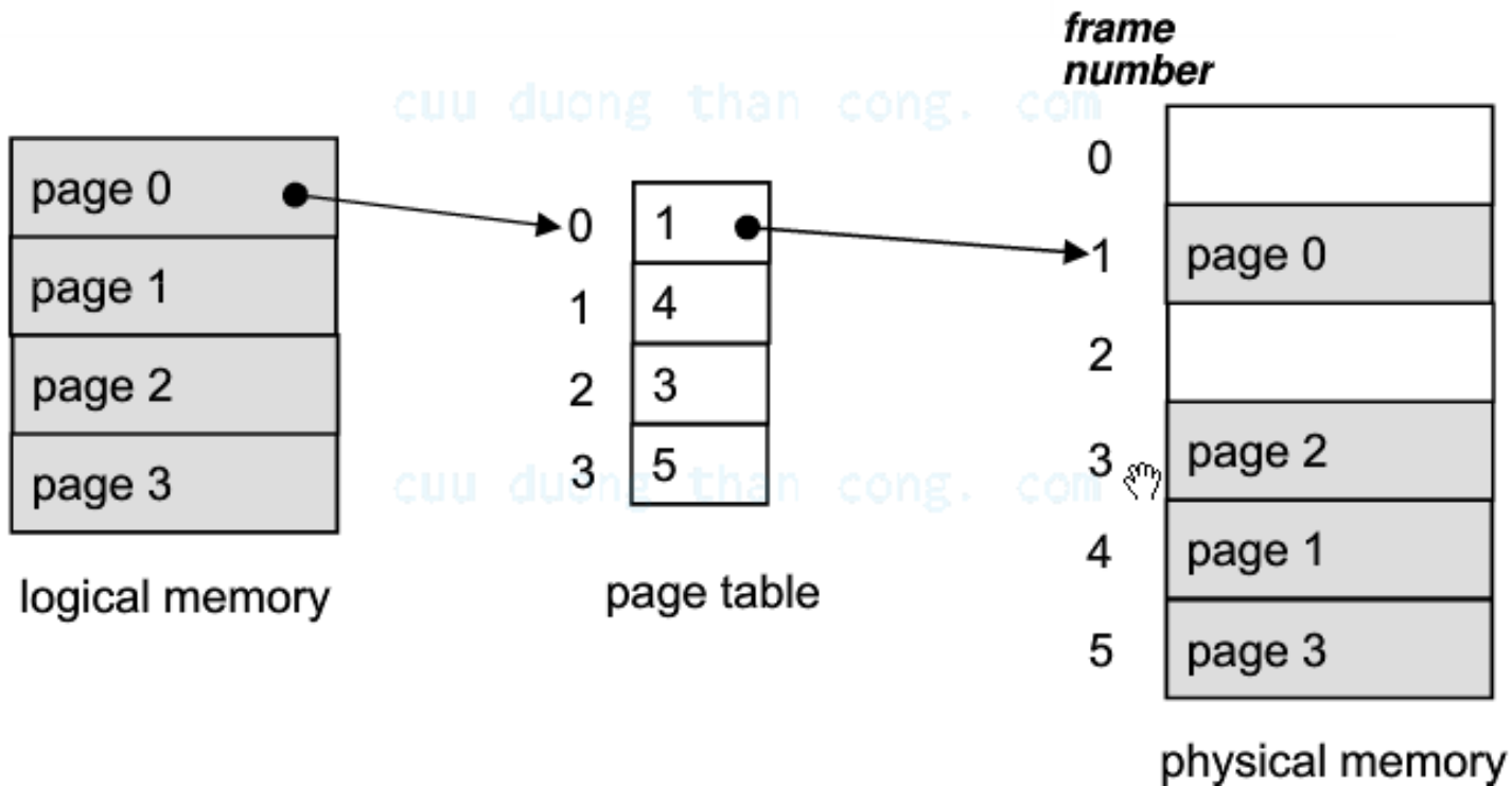
Process D page table
