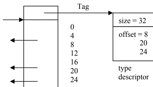
Figure 14.3. Variable with type descriptor.
