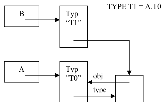
Figure 15.7. Type with aliases.
